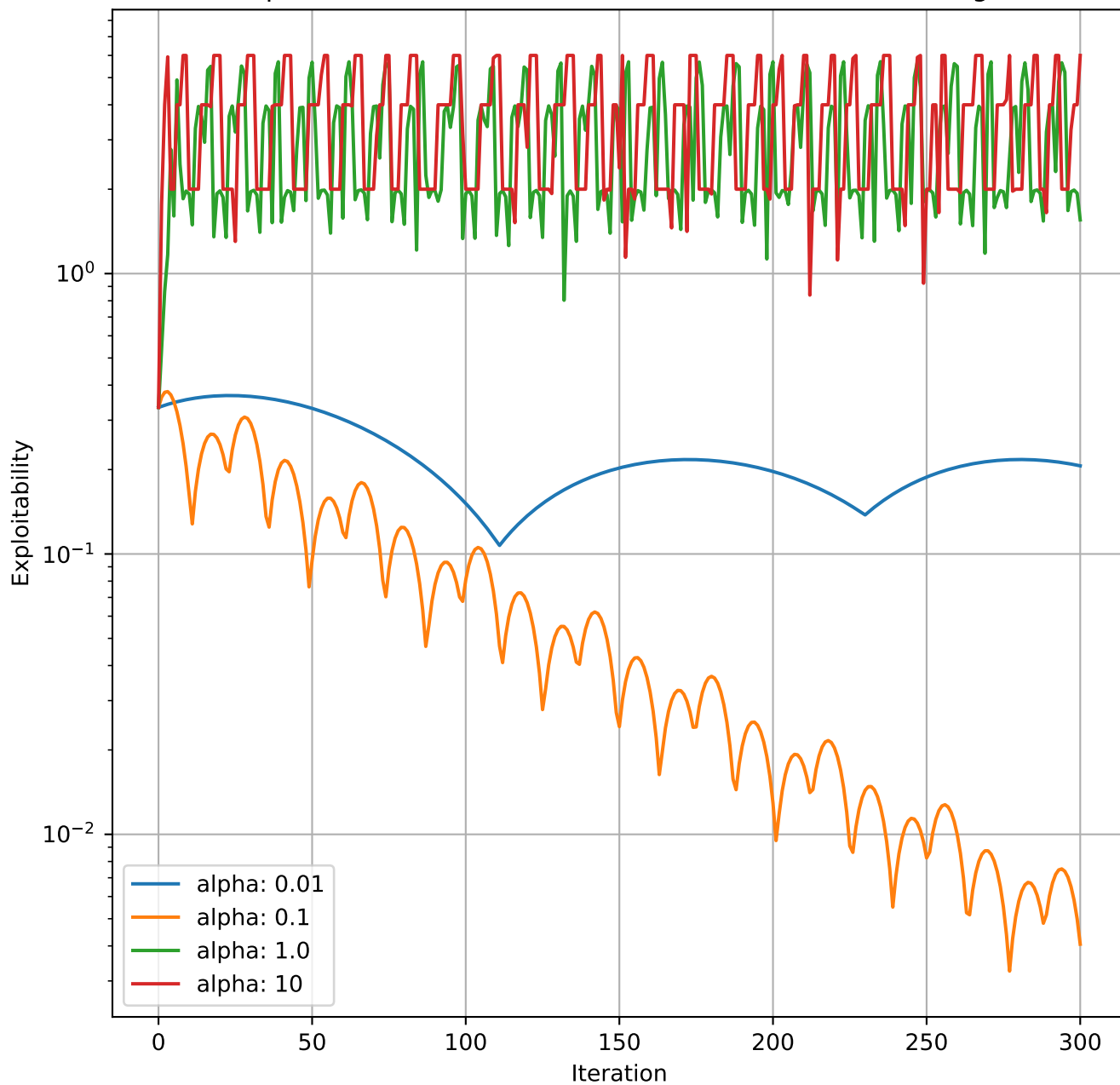
Rock Paper Scissors Environment - Online Mirror Descent Algorithm
