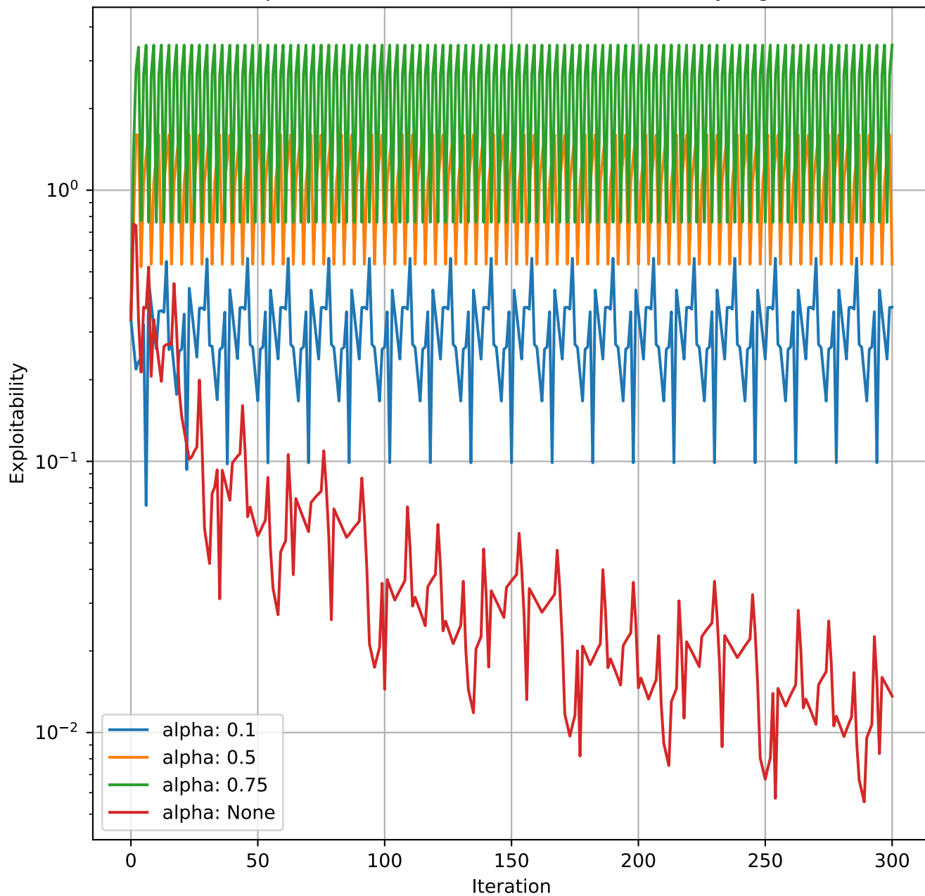
Rock Paper Scissors Environment - Fictitious Play Algorithm
